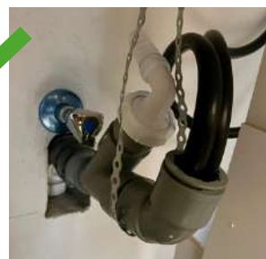
Double-Waste Outlet for Washing Machine + Waste & Overflow for Softener Image 14
